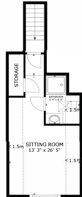
FLOOR 2
